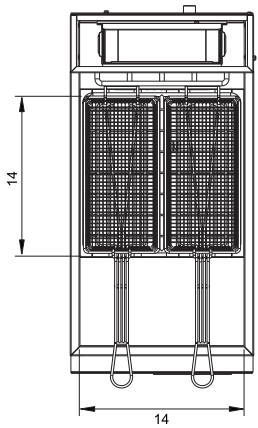
ATFS-40/ ATFS-50
